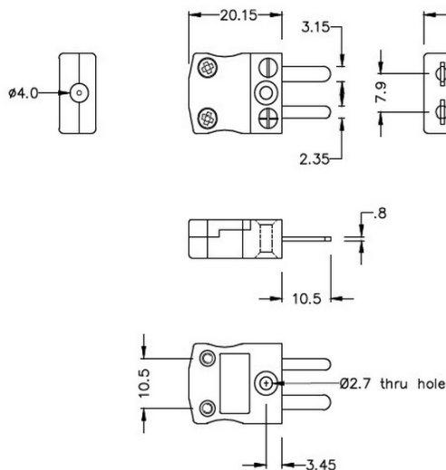
Miniature in-line Plug (dimensions in mm)
